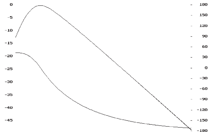
Fig 5. Frequency and phase response of the ELF dual integrator.
