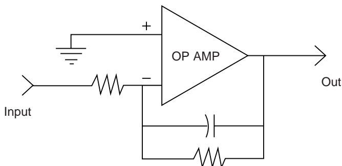
Fig 2. Simple diagram of an integrator.
