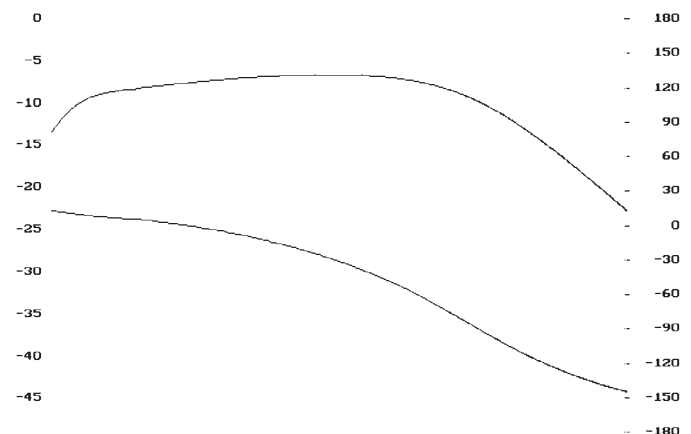
Fig 6. Frequency and phase response of an 80 Hertz low pass filter.
