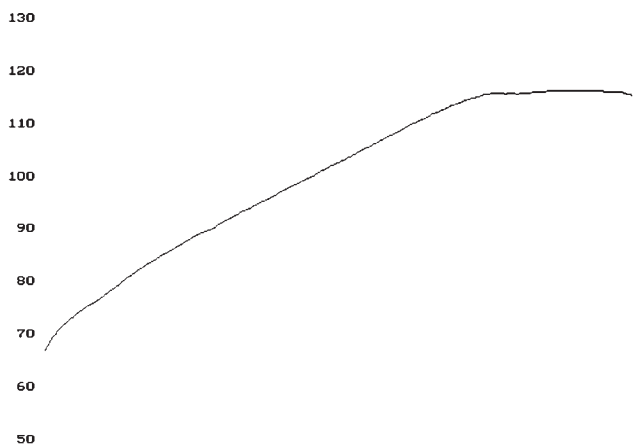
Fig. 17 EL-18 in S18E enclosure dB calibrated to dBSPL. Input signal 28V. (100 watts)
